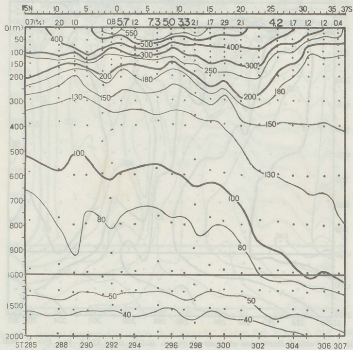
Fig. 6d. Vertical distribution of thermocline anomaly ( \delta\tau , cl/ton), along 55° E-line, Feb. 5-Mar. 9, 1964. Figures along 0 m-line indicate hook rate (%) by the long-line at each station.
