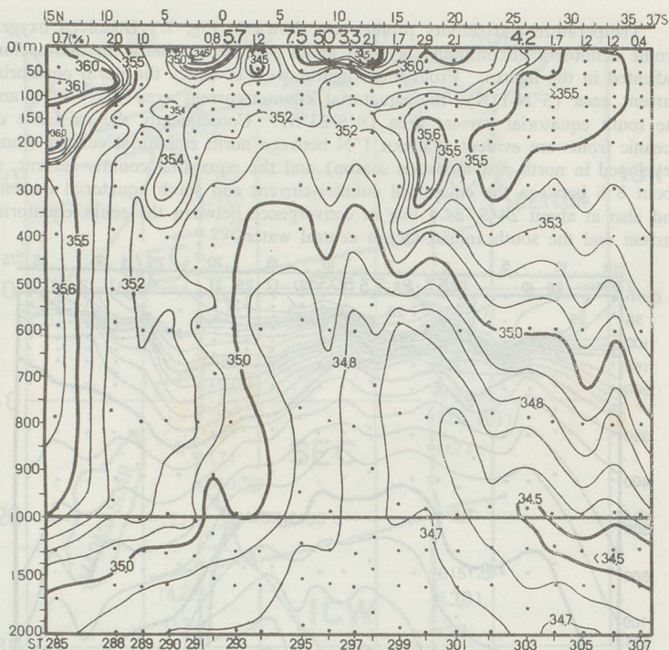
Fig. 6b. Vertical distribution of salinity (‰), along 55° E.-line, Feb. 5-Mar. 9, 1964. Figures along O m-line indicate hook rate (%) by the long-line at each station.
