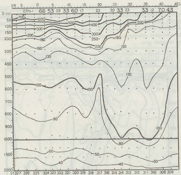
Fig. 7d. Vertical distribution of thermocline anomaly ( \delta\tau , c/ton), along 75°E-line, Apr. 4-30, 1964. Figures along O m-line indicate hook rate (%) by the long-line at each station
