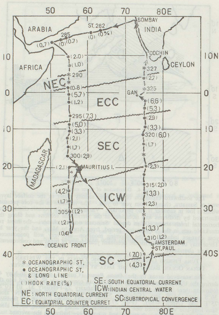
Fig. 5. Cruise track and station positions by the R. V. Anton Bruun Cruise 5, Jan. 26-May 4, 1964. Figures indicate the mean hook rate (%) by the long-line and current system based on data by the R. V. Anton Bruun Cruise 5.
