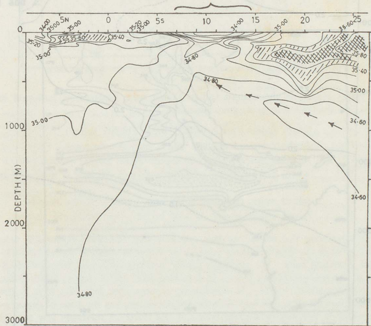
Fig. 1. Vertical distribution of salinity (‰) along the meridional line 78°E (1962/'63)
