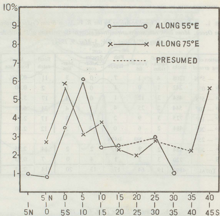
Fig. 9. Arithmetical mean hook rate (%) of Tunas at the intervals of 5° latitude.
