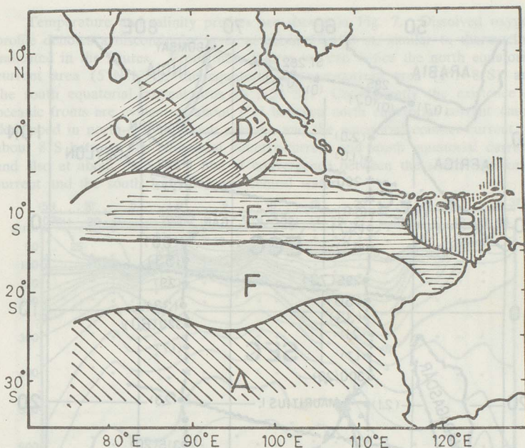
Fig. 4. Distribution of water masses
