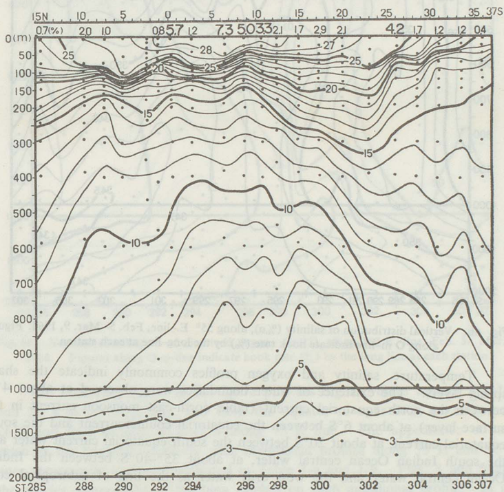
Fig. 6a. Vertical distribution of water temperature (°C), along 55° E.-line, Feb. 5- Mar. 9, 1964. Figures along C m-line indicate hook rate (%) by the long-line at each station. (See Fig. 1)
