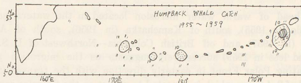
Fig. 26. Distribution of humpback whale catch (1955–1959 accumulated).
