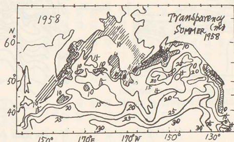
Fig. 13. Transparency in Summer of 1958.
