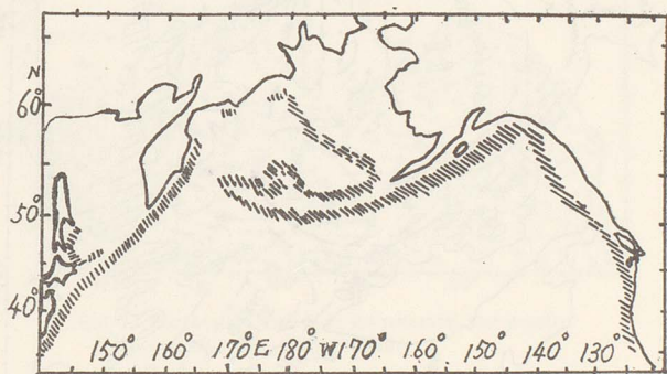
Fig. 1. Zone of maximum bathymetric gradient
