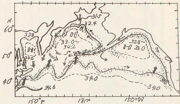
Fig. 9. Oceanic fronts of water masses based on surface salinity (‰), Summer (1955-'58).
