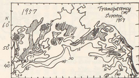
Fig. 12. Transparency in Summer of 1957.
