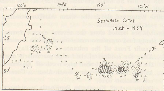
Fig. 25. Distribution of sei whale catch (1955-1959 accumulated).
