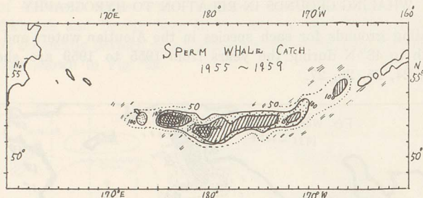
Fig. 24. Distribution of sperm whale catch (1955-1959 accumulated).
