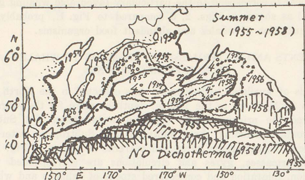
Fig. 4. Dichothermal topography (Summer, 1955~'58)
