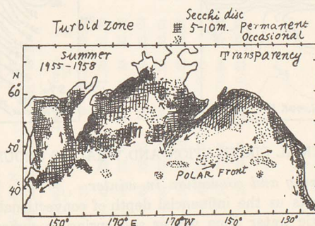
Fig. 14. Distr. of transparency in Summer of 1955~58.
