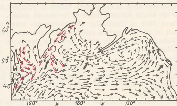
Fig. 3. Circulation based on geopotential topography. Summer (1955-'58) 4D (0/1000 db.)
