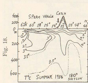
Temp. and salinity sections along Aleutian Islands in contrast to the distr. of sperm whale catch.
