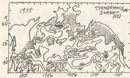
Fig. 10. Transparency in Summer of 1955.
