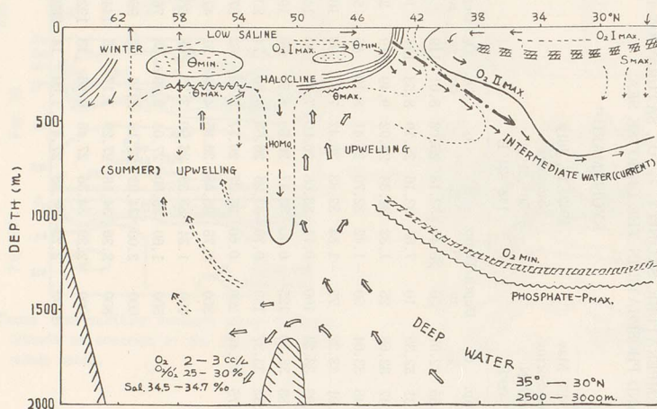
Fig. 22. Schematic circulation pattern in meridional section of North Pacific.
