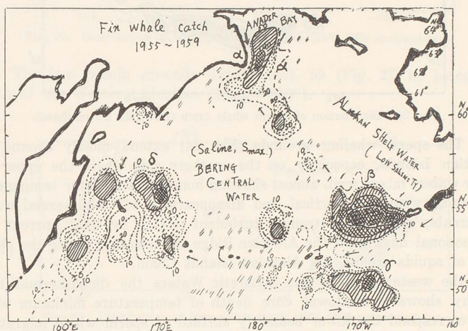
Fig. 23. Distribution of fin whale catch (1955–1959 accumulated).
