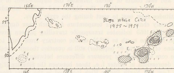
Fig. 27. Distribution of blue whale catch (1955–1959 accumulated).
