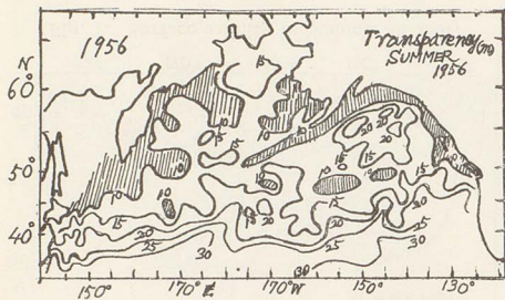
Fig. 11. Transparency in Summer of 1956.
