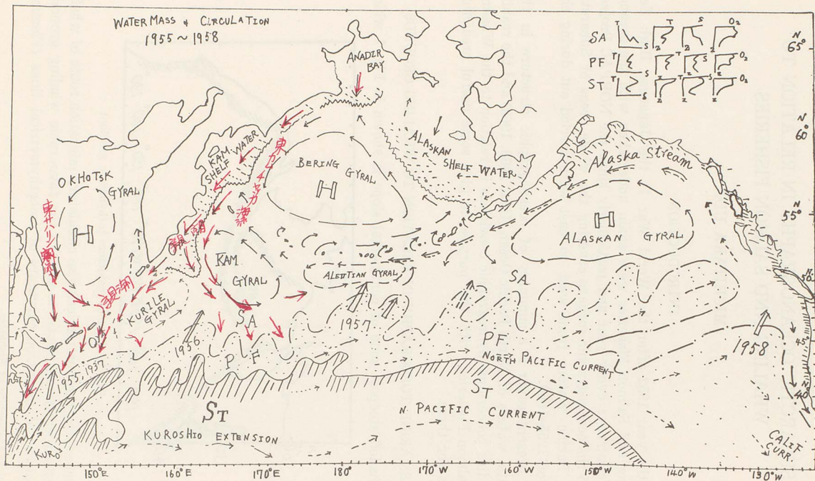
Fig. 2. Schematic map of watermasses and circulation in the Subarctic Pacific (1955-'58).
