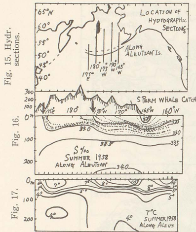
Temp. and salinity sections along Aleutian Islands in contrast to the distr. of sperm whale catch.
