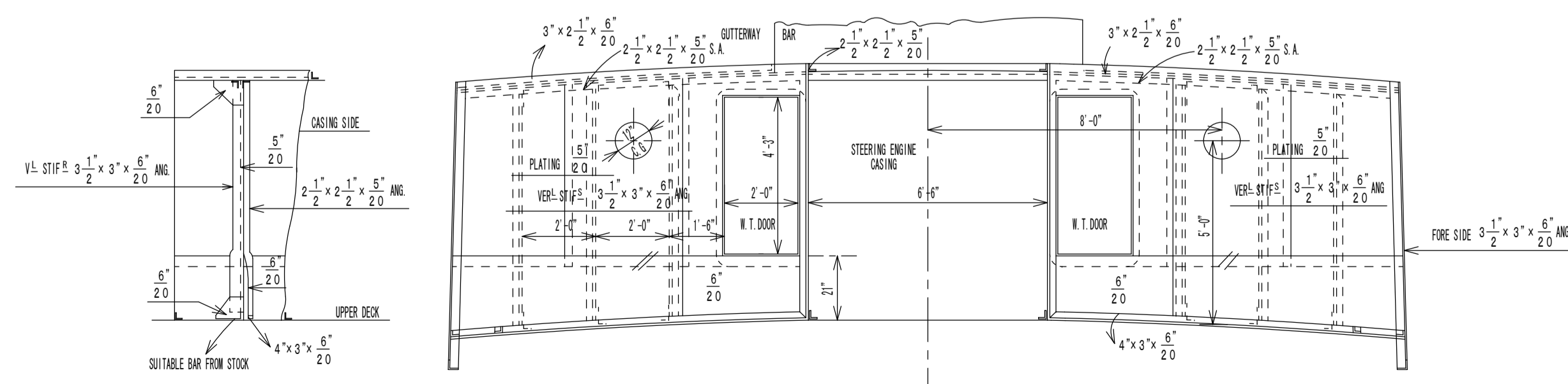
POOP FRONT BULKHEAD. LOOKING AFT.
