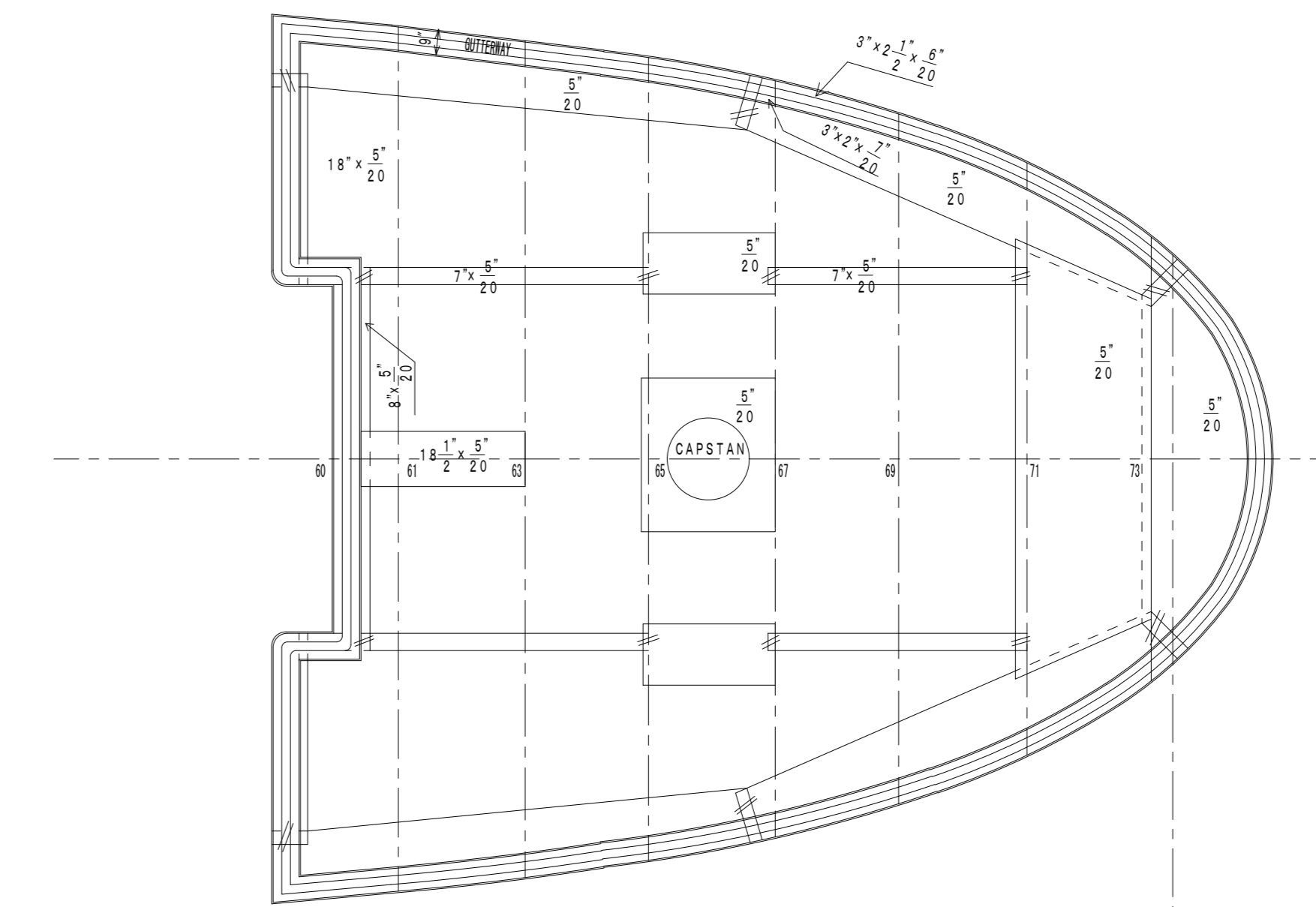
FORECASTLE DECK PLAN
